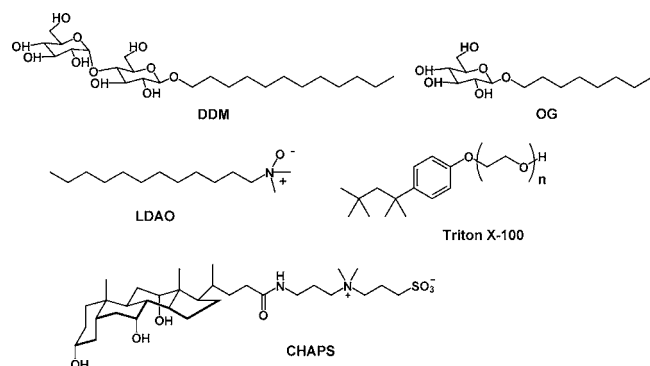
Figure 1. Chemical structures of widely used detergents for membrane protein studies.
